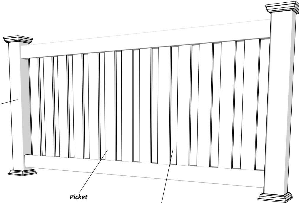
Spacing 50mm
