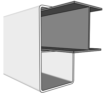
Aluminum profile in top rail to prevent deflection
