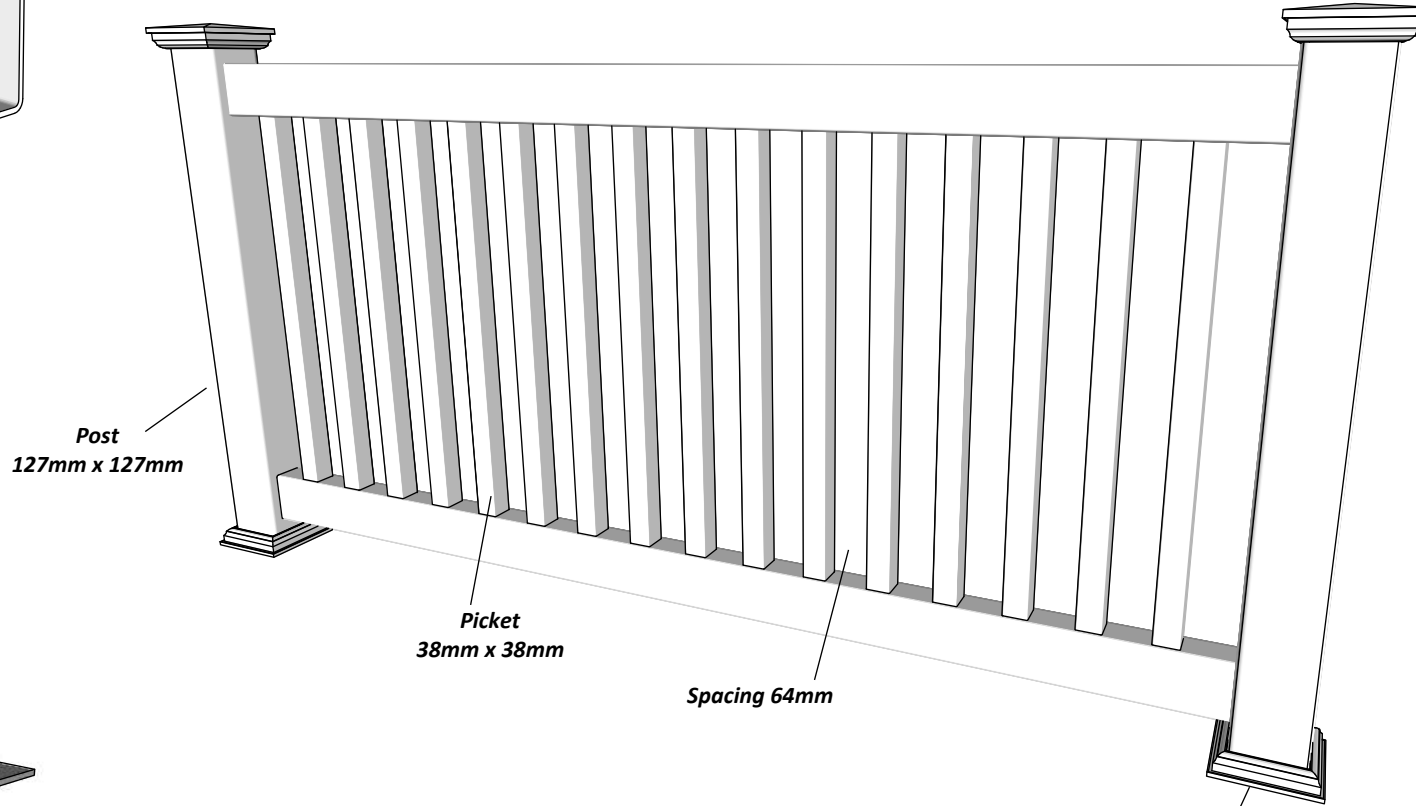
Aluminum profile in bottom rail to prevent deflection
