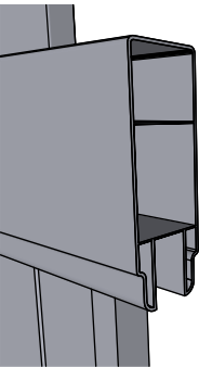
Middle rail profile
