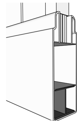
Aluminum profile in bottom rail to prevent deflection
