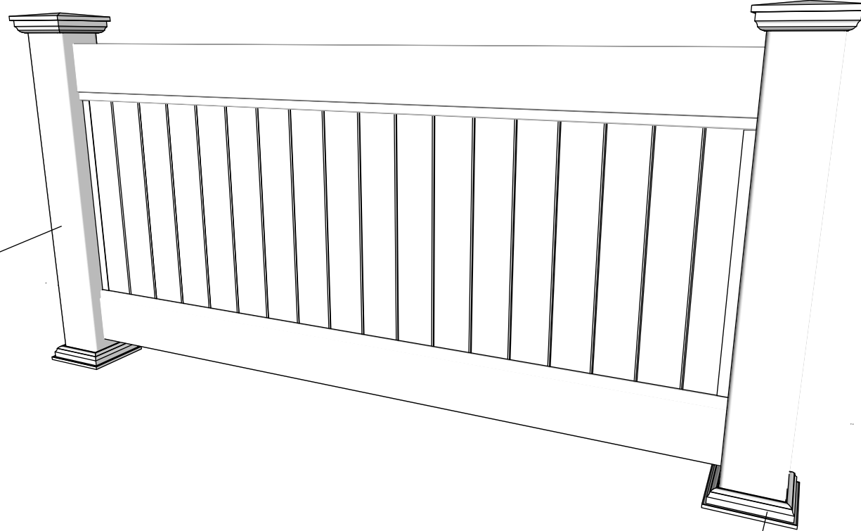
Aluminum profile in bottom rail to prevent deflection
