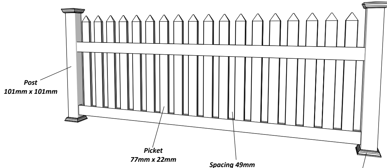
Spacing 49mm
